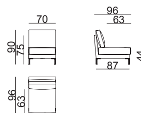
MOD. 70 C/B
