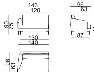
MOD. 120 C/B
