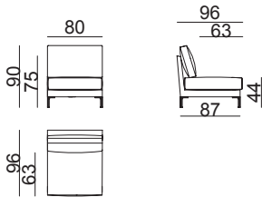
MOD. 80 C/B
